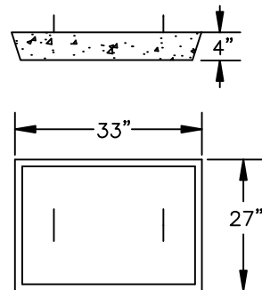
STEEL REINFORCEMENT ROD IN COVER
