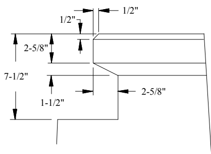
TREAD DETAIL
