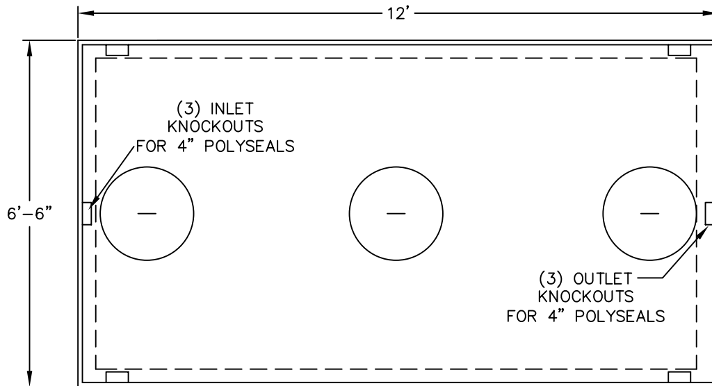
PLAN VIEW
