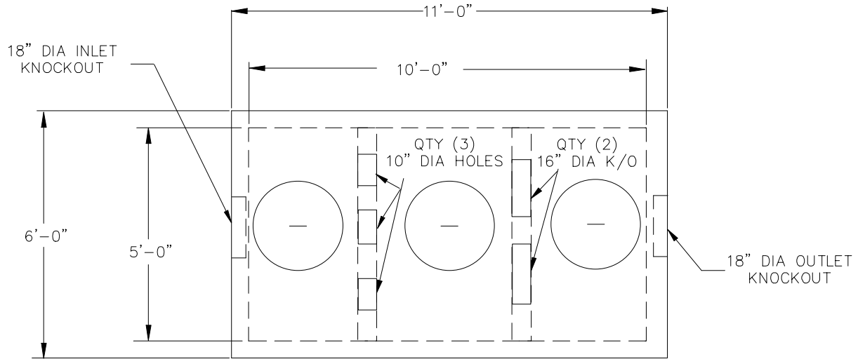
PLAN VIEW
