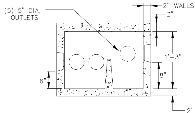
SECTION VIEW
